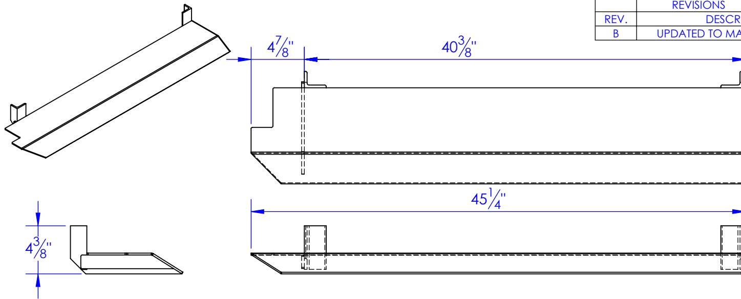
FP-FL95-1 FENDER FLARE, DRIVER, FL-95, WLDMT DRAWING # 90-1214 QTY: 1
